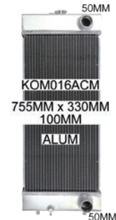
KOMATSU WHEEL LOADER WA200 / WA250
